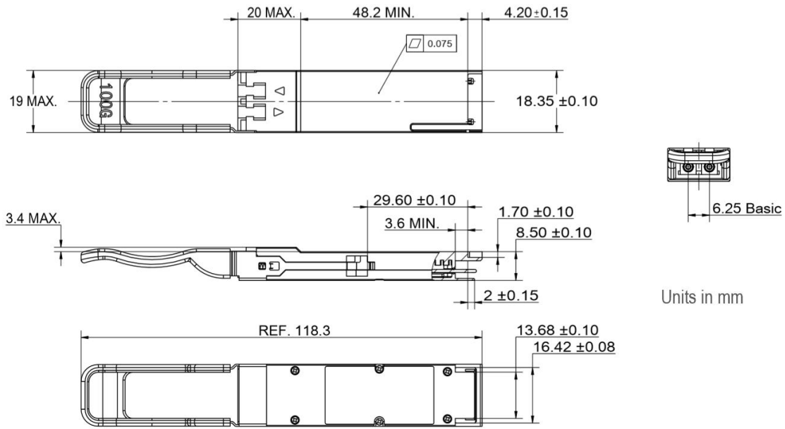
Figure3. Mechanical Outline
